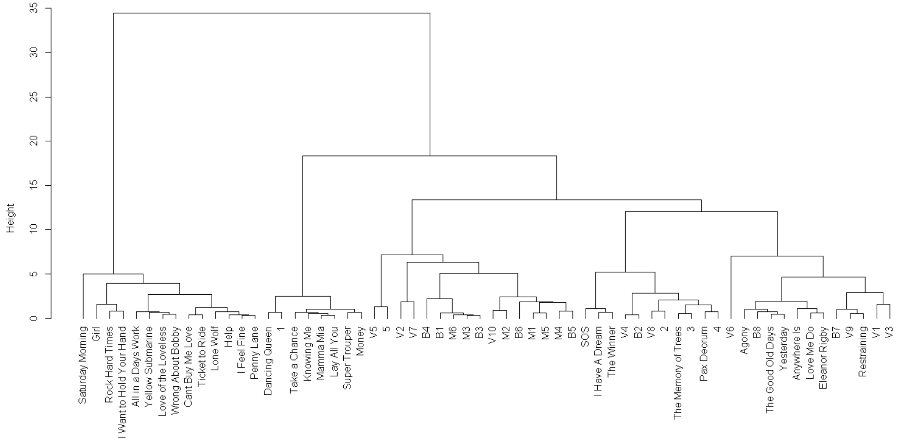
Cluster Dendrogram
