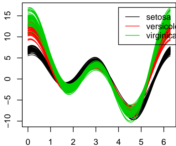
Andrews' Curves
