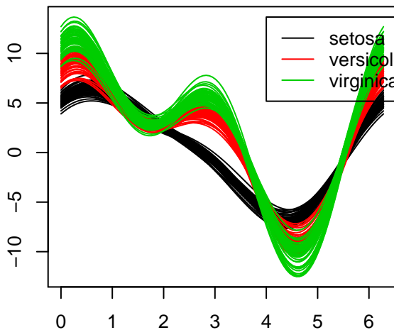
Andrews' Curves
